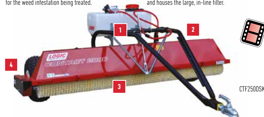
Height adjustment is spring-assisted to allow the machine to be quickly and easily set to the correct working height for the weed infestation being treated.
